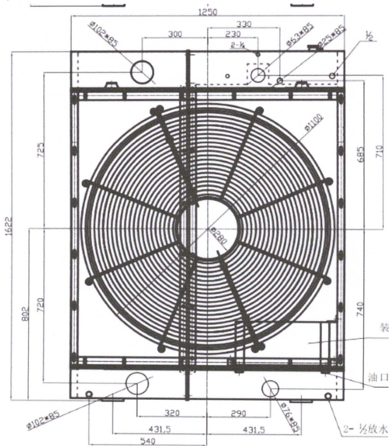
Technical Specification of KTA19-G2 Radiator Assembly
